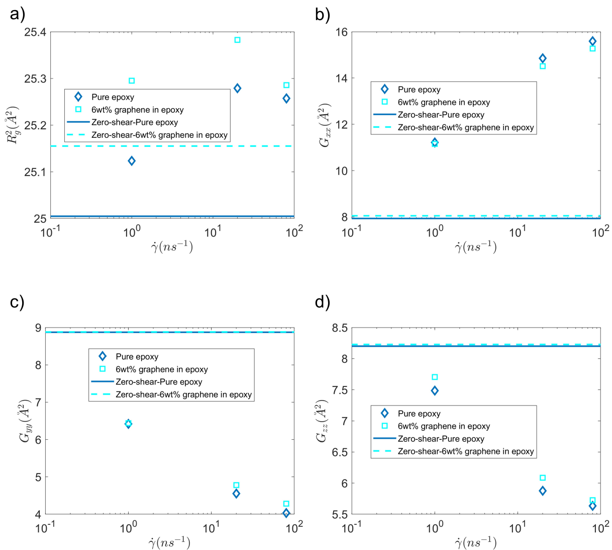
Figure 6. a) Mean-squared radius of gyration, b) G_{xx} , c) G_{yy} and d) G_{zz} of bisphenol F molecules, in pure epoxy and GFI epoxy, in the presence and in the absence of shear slow.
