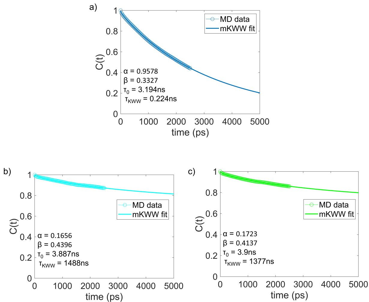
Figure 4. Reorientational correlation function of the end-to-end vectors of a) bisphenol F molecules in pure epoxy and the graphene bound bisphenol F molecules in b) 6wt% graphene infused epoxy and c) 12wt% graphene infused epoxy. The solid lines indicate the mKWW fits [see eq.(5)] for all three cases. The parameters governing the fits for the different cases have been provided in each of the figures.
