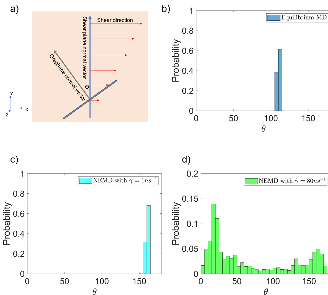
Figure 7. Probability distribution of the angle [shown schematically in (a)] between the graphene normal vector and the y-axis (normal vector to the shear planes in NEMD simulations) in the b) absence and c, d) presence of shear flow for the case of 6wt% graphene infused epoxy system.
