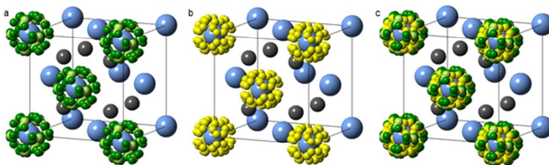
Figure 2 – The cubic structural models used for a) lithium amide b) lithium imide and c) the combined lithium imide-amide structure. Lithium atoms are shown in dark grey, nitrogen in blue, and deuterium in light and dark green for the amide positions, and yellow for the imide positions. For clarity, deuterium positions are only indicated for those bonded to the front face of nitrogen atoms.
