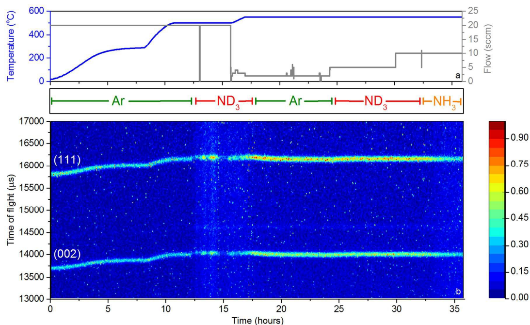
Figure 5 – Neutron powder diffraction experiment, showing a) reaction conditions: temperature (blue) and gas flow set point (grey), along with the input gas species listed below, and b) a contour plot of the neutron diffraction data showing the (111) and (002) reflections of \text{Li}_2\text{ND} . The colour bar to the right gives an indication of the scattering intensity.
