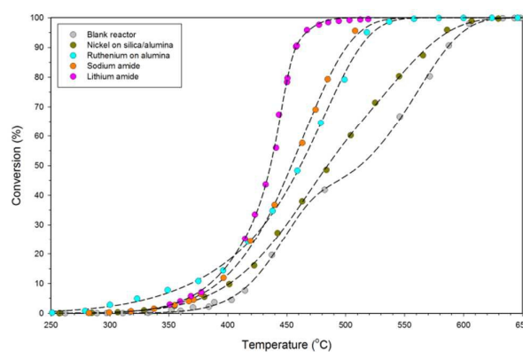
Figure 3 – Comparison of ammonia conversion as a function of reaction temperature (between 250 and 650 °C) for the blank 46.9 cm 3 stainless steel reactor and when containing 0.5 g of LiNH 2 , NaNH 2 , silica/alumina-supported nickel, and alumina-supported ruthenium, at an ammonia flow rate of 60 sccm, with dashed lines showing sigmoidal fits to the data.
