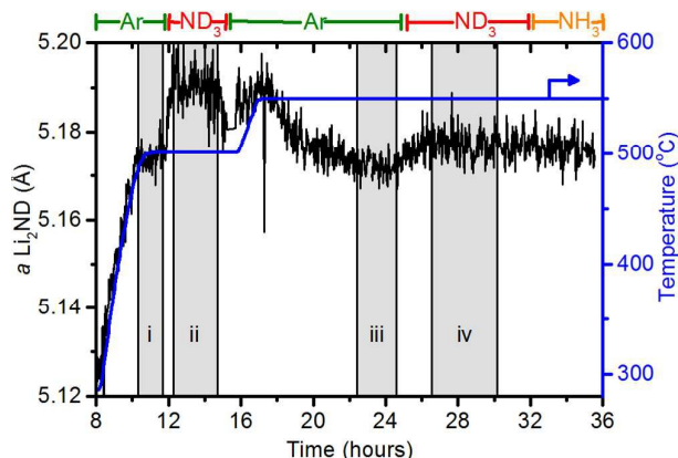
Figure 6 – Variation of the a lattice parameter of \text{Li}_2\text{ND} (black) over the course of the experiment. The temperature of the sample (blue) is shown for comparison. Shaded areas represent periods of NPD data which were summed and analysed for the sample stoichiometry.
