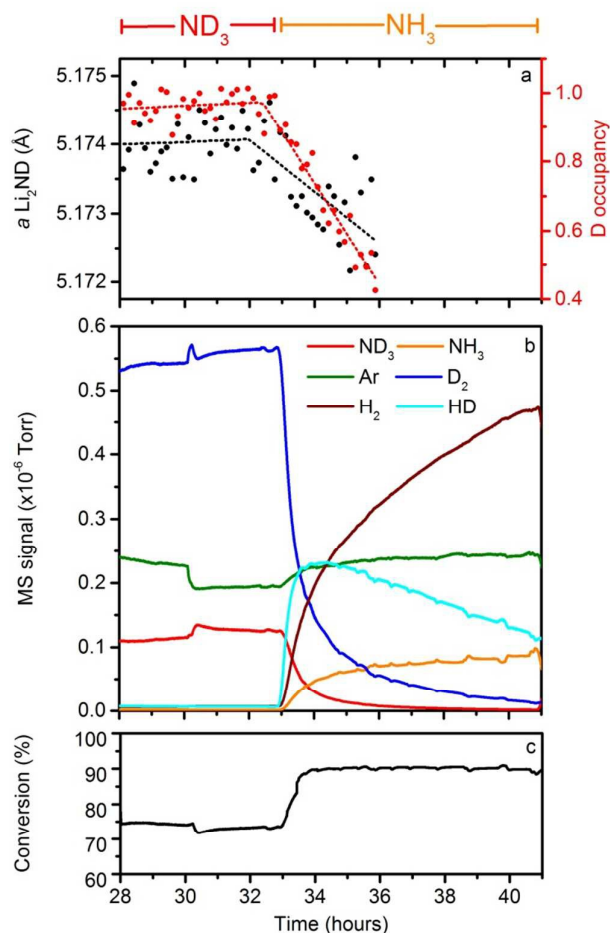
Figure 7 - H-D exchange experiment, where the gas species flowing across the sample during the experiment are shown at the top. The panels show a) the refined deuterium occupancy (red) and lattice parameter (black) in the \text{Li}_2\text{ND} sample, b) the QGA data collected during the experiment and c) the ammonia conversion percentage data.
