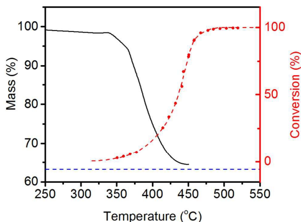
Figure 4 – Thermogravimetric analysis data showing the decomposition of \text{LiNH}_2 under ammonia (black), compared with the ammonia decomposition efficiency data under 60 sccm ammonia flow (red) and a sigmoidal fit to the decomposition data (dashed red). The expected mass loss for decomposition to \text{Li}_2\text{NH} is shown as a dashed blue line.
