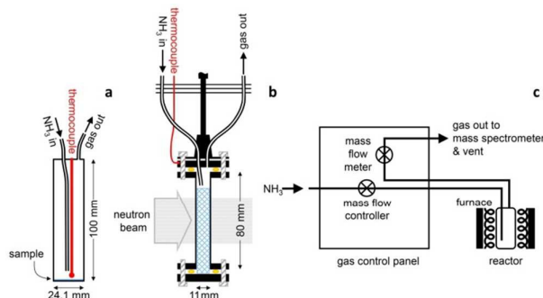
Figure 1 – Reactor and experimental set-ups: (a) A typical 46.9\text{ cm}^3 reactor showing NH_3 inlet, gas outlet, and thermocouple temperature probe positions, with a 0.5 g sample, drawn to scale. (b) The analogous in situ neutron diffraction set-up highlighting the powder sample contained within a 0.35 mm wall thickness stainless steel cell and held in position in the neutron beam. (c) Experimental gas handling set-up, where the inlet NH_3 gas flow is controlled prior to the reactor, and the outlet gas flow is monitored by a mass flow meter and analysed by a mass spectrometer.
