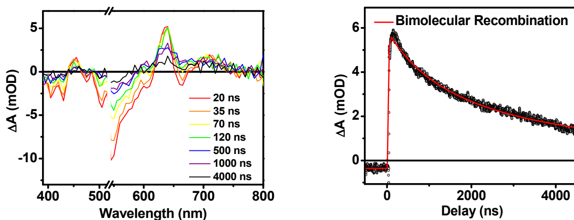
Figure 7. Nanosecond transient spectra of an annealed film of 1 (left) and its transient kinetic trace at 645 nm (right). The nsTA data (black points) is fit using a bimolecular decay (red line).
