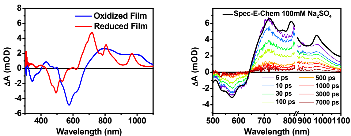
Figure 4. (Left) A comparison of spectroelectrochemical difference spectra of 1 electrochemically oxidized and reduced in a film on ITO. (Right) a comparison of the sum of the reduced and oxidized species spectra to the fsTA spectrum of an unannealed film of 1 .
