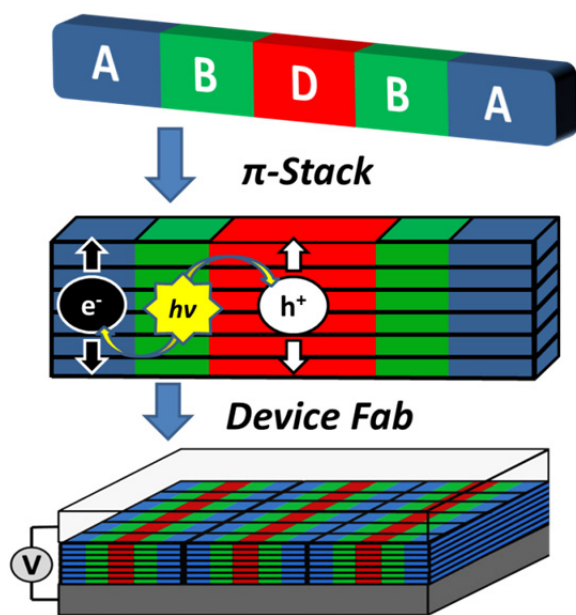
Figure 1. Cartoon depicting the self-assembly of a covalent donor-bridge-acceptor (D-B-A) system to control charge separation and form segregated electron and hole conducting pathways.
