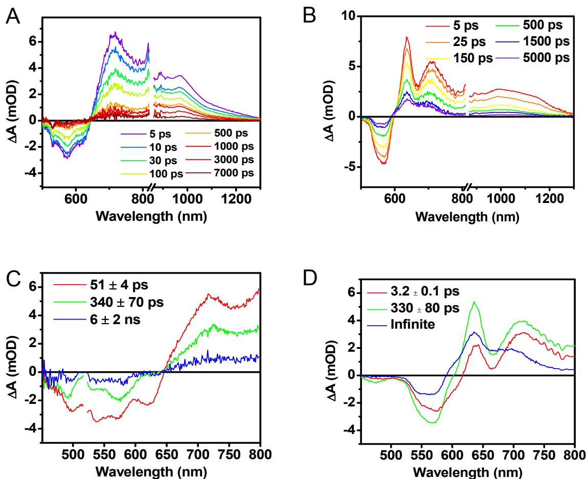
Figure 6. fsTA spectra of an as cast, unannealed thin film of 1 (A), and a film that was solvent vapor annealed for ten minutes with \text{CH}_2\text{Cl}_2 (B). Singular value decomposition (SVD) and global fitting gave decay associated spectra for the unannealed (C) and annealed (D) films.
