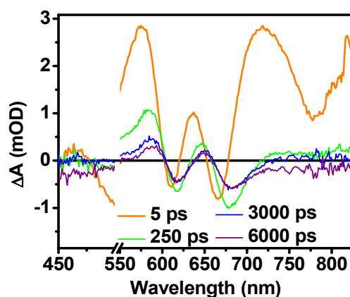
Figure 8. FsTA spectra of a film of 2 that has been solvent vapor annealed for 10 minutes in \text{CH}_2\text{Cl}_2 showing positive absorptions at 580 and 650 nm resulting from ^3\text{DPP} formation.
