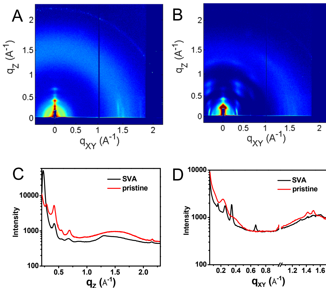
Figure 3. GIWAXS of a pristine (A) film of 1 and a film which has been solvent vapor annealed in \text{CH}_2\text{Cl}_2 for 10 min (B) as well as vertical (C, q_{xy} = 0 ) and horizontal (D, q_z = 0 ) line cuts of the annealed (black) and unannealed (red) films.
