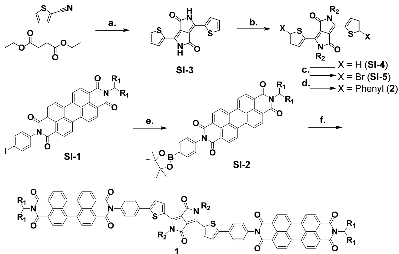
Scheme 1. Synthesis of molecules 1-2 . a
