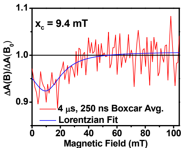
Figure 10. Relative transient absorption intensity of 1 films vs. magnetic field measured at 635 nm and 4.0 \mu\text{s} after a 7 ns, laser pulse..
