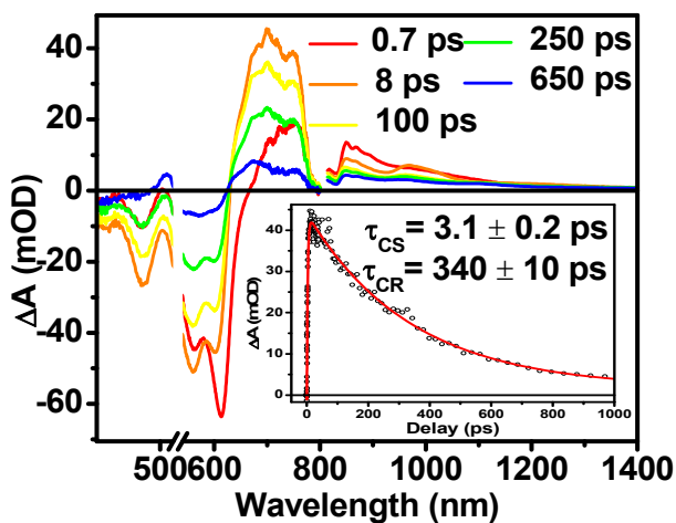
Figure 5. fsTA spectra of 1 in toluene. Inset shows the kinetics and fit of the data at 700 nm.
