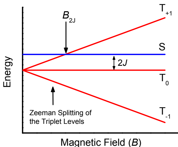
Figure 9. Schematic of radical ion pair energy levels as a function of magnetic field for J > 0 .
