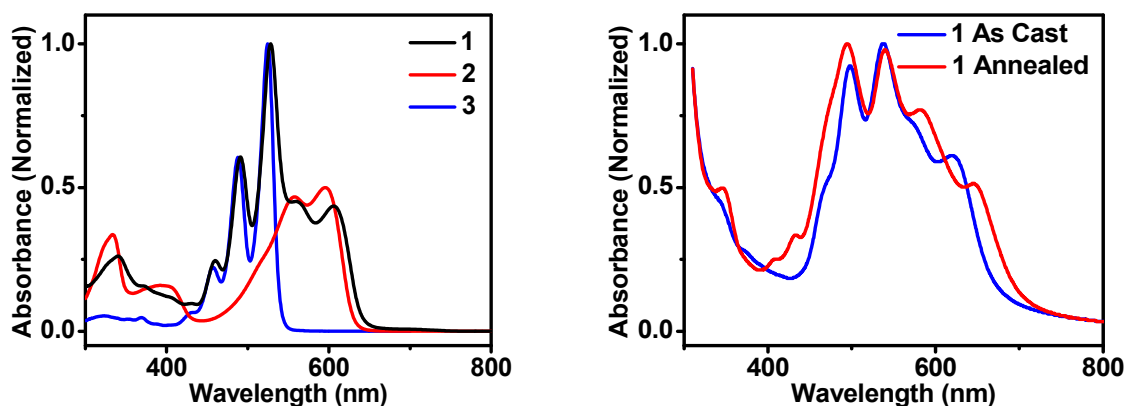
Figure 2. UV-visible absorption spectra of molecules 1 , 2 , and 3 in toluene solution (left), and of thin films of 1 that are unannealed and \text{CH}_2\text{Cl}_2 vapor annealed for 10 minutes (right).
