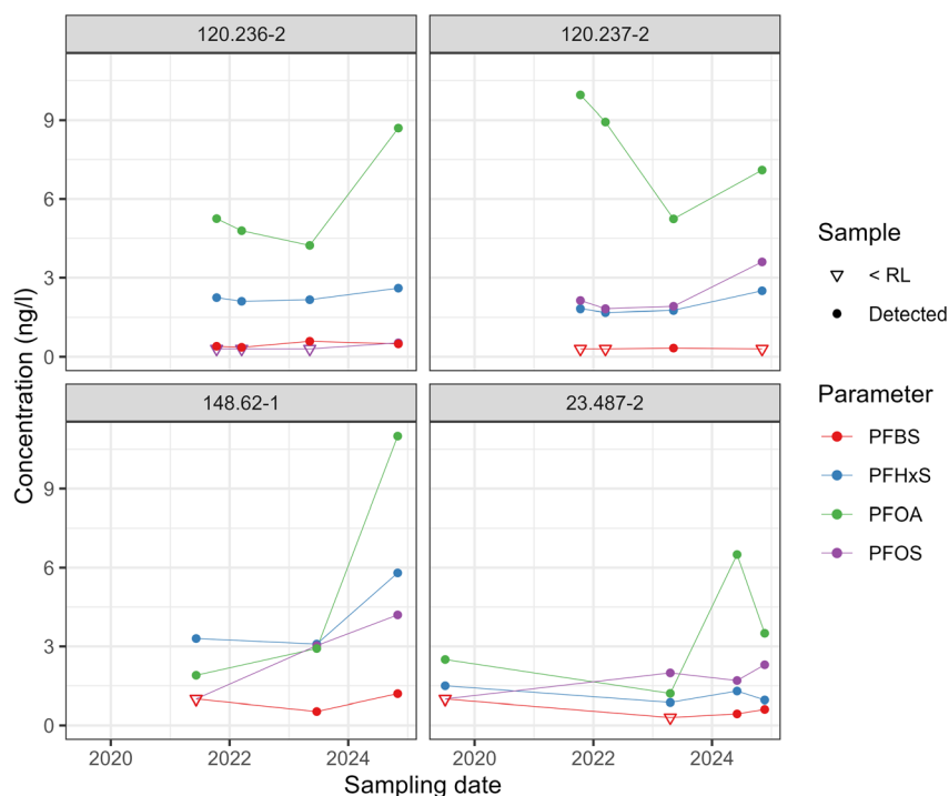
Fig. 4 Time series for repeatedly detected PFAS compounds in four wells with the sea spray aerosols from the North Sea as the suspected source. Further details of the individual wells are shown in Table 1. Open triangles denote that the compound was not detected at that sampling date with the concentration depicting the Reporting Limit (RL) of that analysis.
