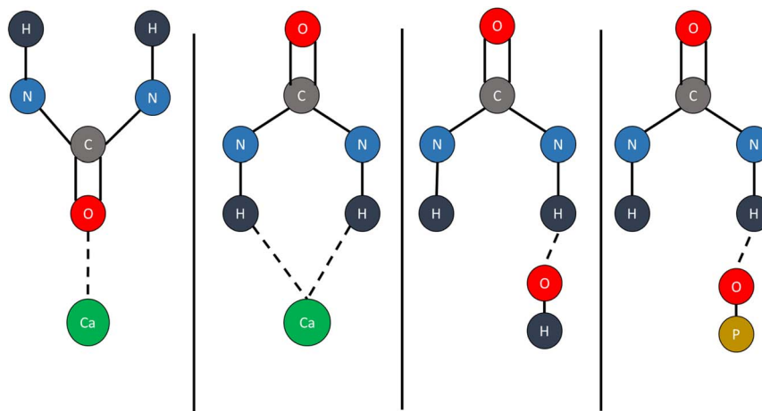
Fig. 4 Proposed bonding modes between \text{Ca}^{2+} , \text{O}_3-\text{PO}_4^{3-} , and \text{OH}^- in HAP with -\text{CO}- and \text{NH}- functional groups of urea. 35 Assignments were made based on previous literature reports using metal-urea complexes.
