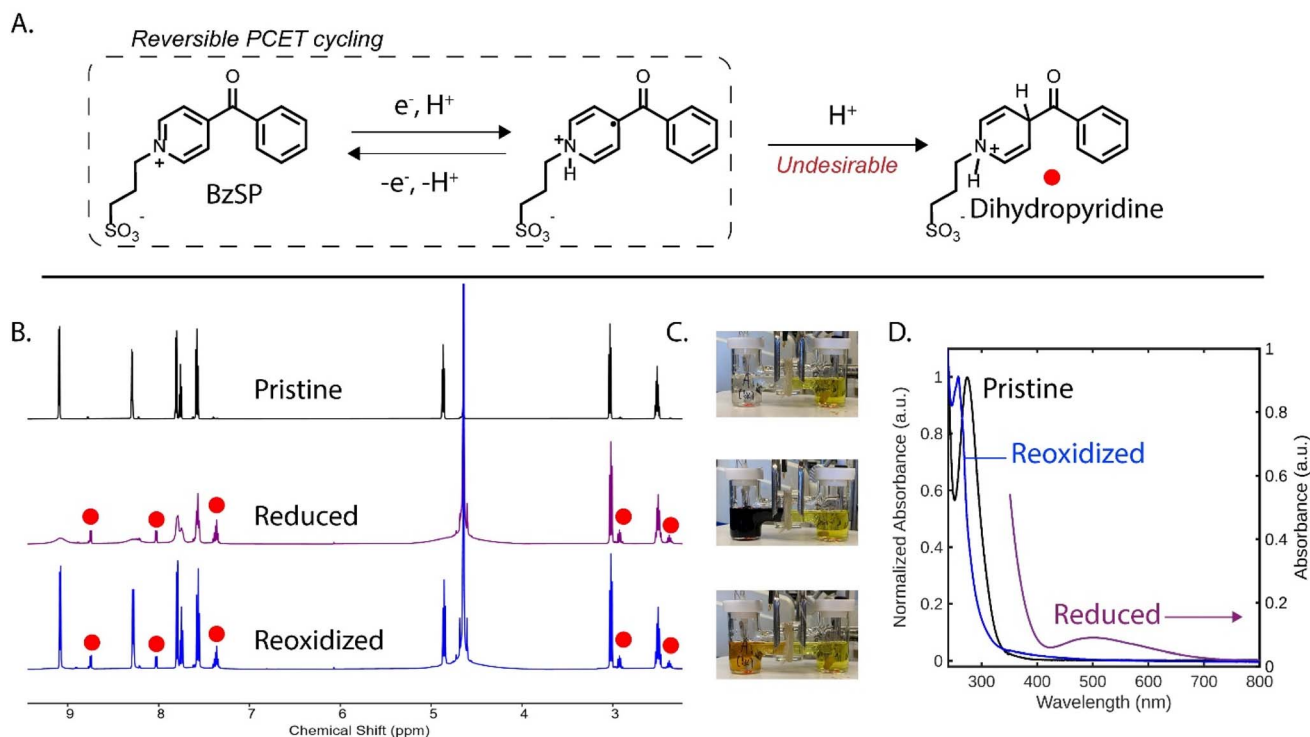
Fig. 5 (A) Mechanism for BzSP-mediated CO 2 capture, including degradation reaction to dihydropyridine. (B) ^1H NMR spectra ( D_2O , 500 MHz) of 0.1 M BzSP in 1 M KNO_3 at different stages of the cycling process. (C) Photographs of the BzSP solution (left compartment) at each stage. (D) UV-visible absorption spectra at each stage. The pristine and reoxidized spectra are normalized, while the reduced spectrum is not. A large absorbance below 400 nm in the reduced spectrum is due to the high concentration of active species, which is necessary to observe the radical band.
