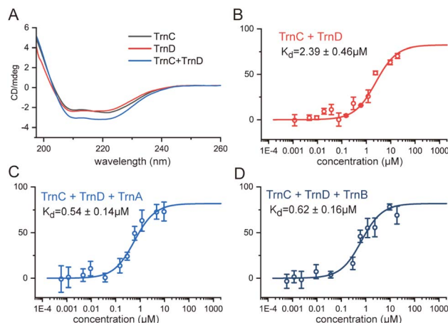
Fig. 4 TrnC and TrnD form a stable protein complex. Formation of a robust protein complex between TrnC and TrnD in thuricin CD biosynthesis, showing (A) CD spectra of TrnC, TrnD, and a 1 : 1 mixture of TrnC and TrnD, and MST analyses of the fluorescently labeled TrnC with (B) TrnD, (C) TrnD and TrnA, and (D) TrnD and TrnB.
