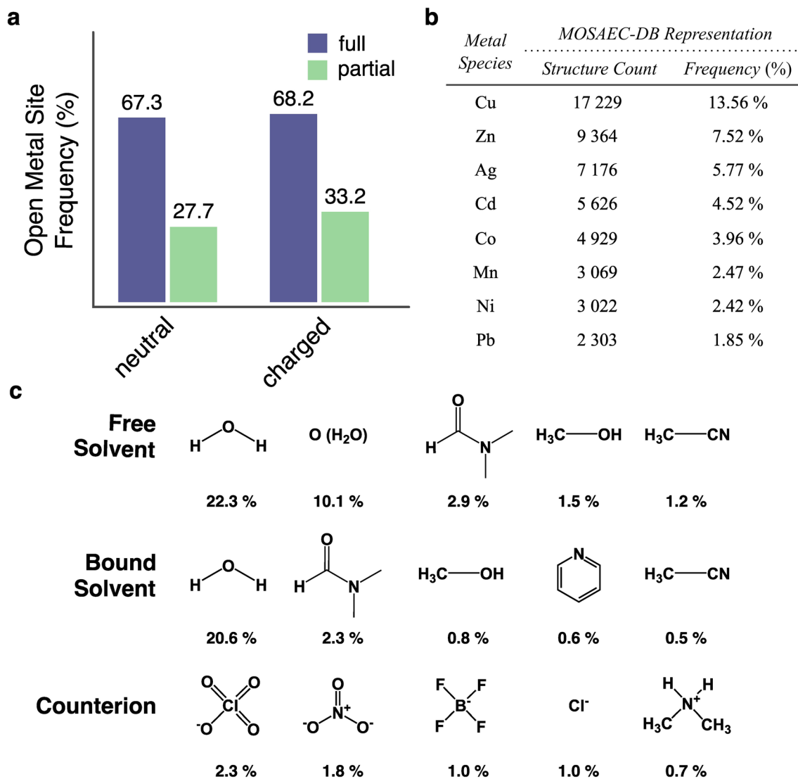
Fig. 5 Survey of the open metal site (OMS) and solvent removal statistics observed in the processed MOSAEC-DB MOFs, including: (a) frequency of OMS across the activation state and framework charge subcategories, (b) most common OMS species by metal identity, and (c) most common free solvent, bound solvent, and counterions removed during solvent processing.
