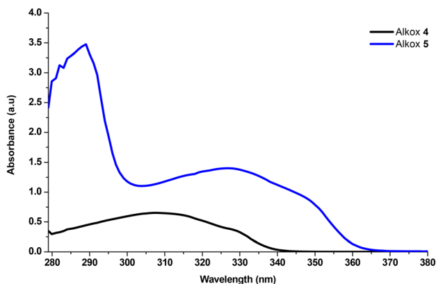
Fig. 1 UV – Visible spectra overlay of bromo tacrine-based alkoxyamine 4 and D- \pi -A tacrine TMO-based alkoxyamines 5 in tert -butyl benzene with concentration = 1.0 \times 10^{-4} M.
