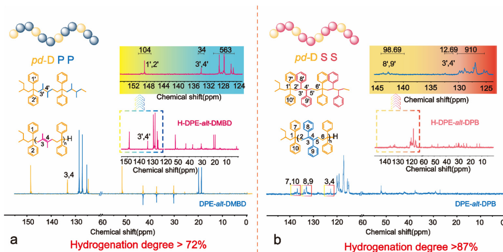
Fig. 3 IG- ^{13}\text{C} NMR spectra of alternating polymers and periodic polymers: (a) for the copolymer of DPE with DMBD and (b) for the copolymer of DPE with DPB.
