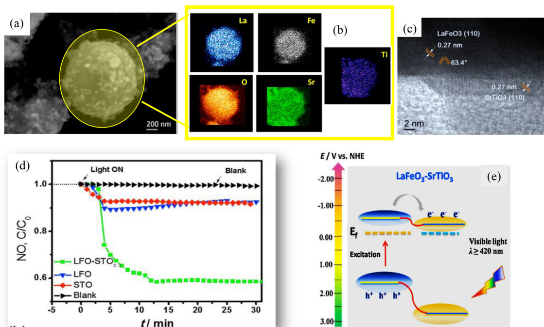
Fig. 5 (a) Representative scanning electron microscopy (SEM) image and (b) the corresponding EDX chemical maps for a LaFeO 3 -SrTiO 3 heterostructured system, obtained by ultrasonic spray pyrolysis, followed by solvothermal treatment. (c) HR-TEM image of the LFO/STO interface. (d) Photocatalytic NO removal profiles ( C/C_0 ) as a function of time (Vis-light irradiation). (e) Schematic band energy diagram for LFO-STO heterostructures and the corresponding charge carrier separation under Vis illumination. Reprinted with permission from ref. 12. Copyright 2017, Elsevier.
