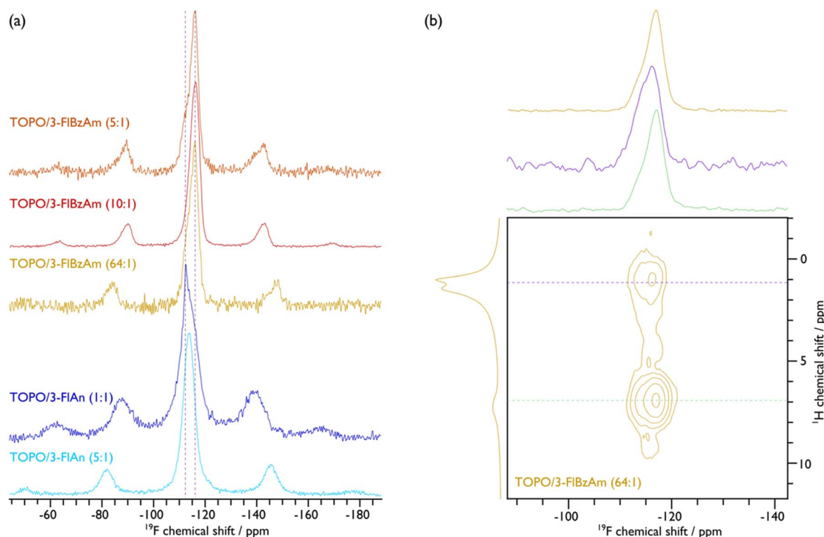
Fig. 5 \{{}^1\text{H}\}\text{-}{}^{19}\text{F} CP (a) and {}^1\text{H}\text{-}{}^{19}\text{F} 2D dipolar correlation (b) MAS NMR spectra of indicated CdS NCs. An MAS frequency of 10 kHz was used for TOPO/3-FIAn (1 : 1), TOPO/3-FIBzAm (10 : 1), and TOPO/3-FIBzAm (5 : 1), and 12 kHz was used for TOPO/3-FIAn (5 : 1) and TOPO/3-FIBzAm (64 : 1) CdS NCs. Cross-sectional slices at the positions indicated with the horizontal dashed coloured lines in the 2D spectrum are given above the 2D spectrum in (b) along with the corresponding \{{}^1\text{H}\}\text{-}{}^{19}\text{F} CP (top) and {}^1\text{H} (left) MAS NMR spectra. See the ESI† for corresponding spectral fittings.
