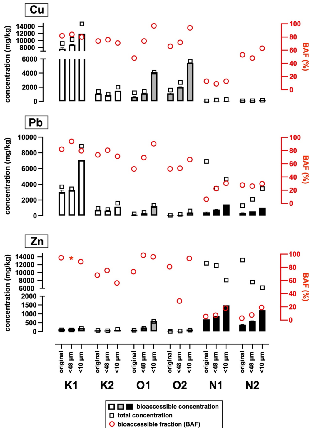
Fig. 3 Total concentrations (squares), bioaccessible concentrations (bars), and bioaccessible fractions (red dots) of Cu, Pb, and Zn in the original tailings and the <48 \mu\text{m} and the <10 \mu\text{m} fractions of the tailings. Asterisk indicates an outlier BAF value for Zn, exceeding 100%, probably related to the “nugget effect” and/or sample inhomogeneity. Symbols for the individual sites: K = Kombat, O = Oamites, N = Namib Lead & Zinc.
