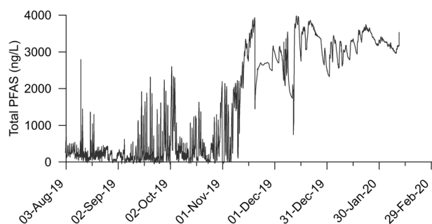
Fig. 5 Estimated concentration of total PFAS ( \sum \text{SC} + \text{LC} + \text{USC} ) for epibenthic exposure within the HB pond plume footprint, based on continuous SpC measurements at \sim 1 \text{ cm} above the pond sediments.
