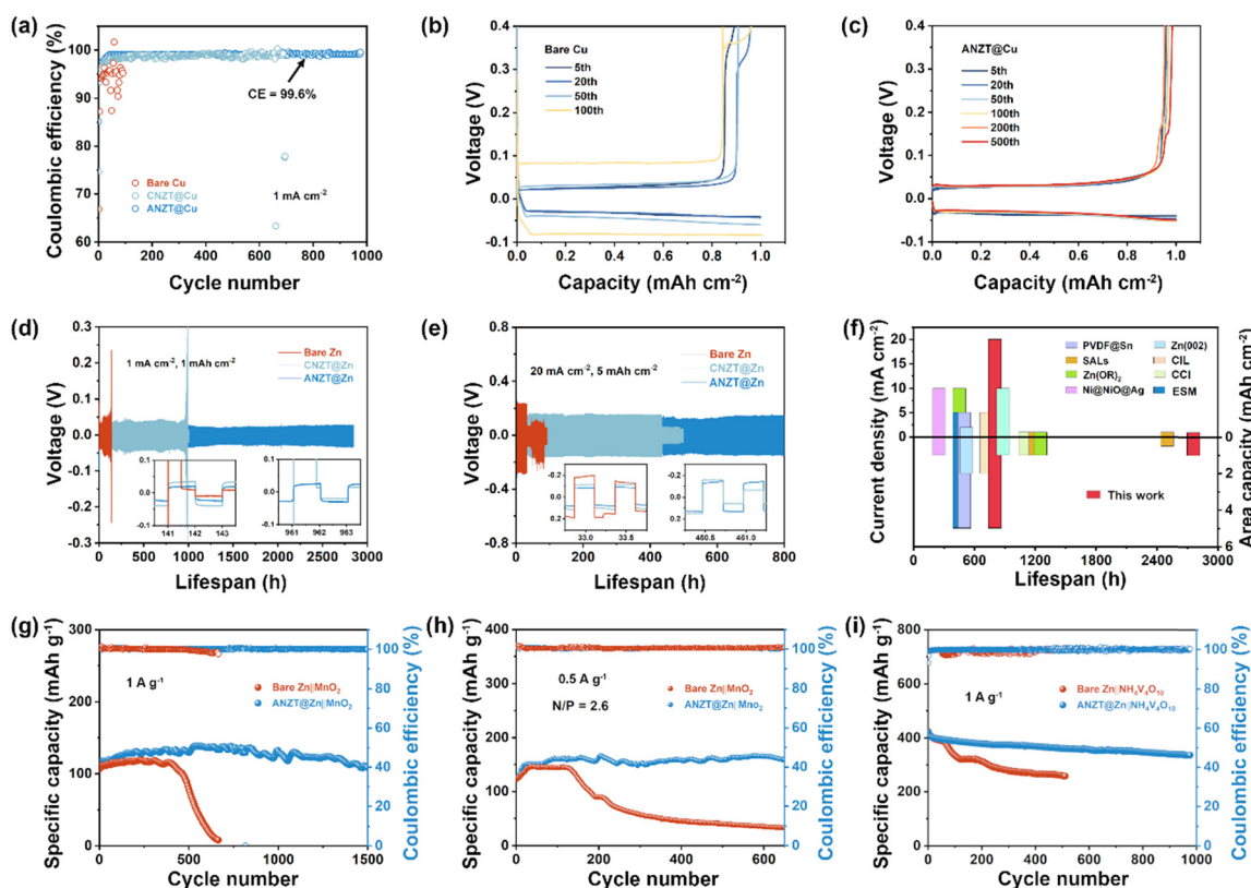
Fig. 3 (a) CE test of the Zn||Cu half-cells with bare Cu, CNZT@Cu, and ANZT@Cu electrodes (1 mA cm -2 /1 mA h cm -2 ). Charge–discharge curves of the Zn||Cu half-cells with (b) bare Cu and (c) ANZT@Cu electrodes at the 5th, 20th, 50th, 100th, 200th, and 500th cycles, respectively. Cycle performance of the Zn||Zn symmetric cell cycled at a current density of (d) 1 mA cm -2 with a capacity of 1 mA h cm -2 and (e) 20 mA cm -2 with a capacity of 5 mA h cm -2 . (f) Comparison of the cyclic lifespan of the ANZT@Zn anode with recently reported anode-modified strategies. Cycling performance of the Zn||MnO 2 cells at the current densities of (g) 1 A g -1 and (h) 0.5 A g -1 (10 μm Zn foil, with a low N/P ratio of 2.6). (i) Cycling performance of the Zn||NH 4 V 4 O 10 cells with bare Zn and ANZT@Zn anodes at a current density of 1 A g -1 .
