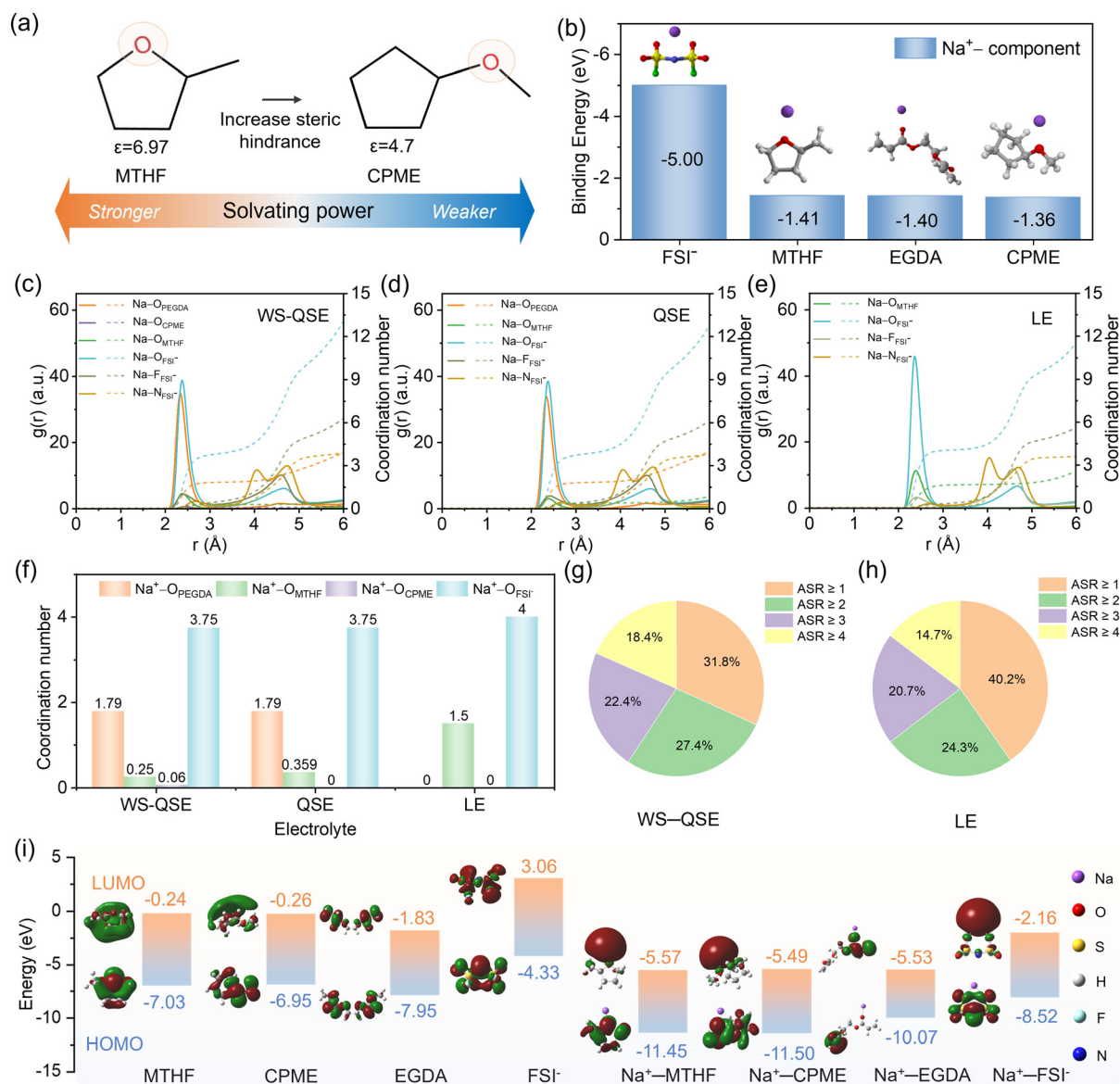
Fig. 2 (a) Molecular structure of MTHF and CPME with an illustration of solvating power. (b) Binding energies of \text{Na}^+ -FSI ^- , \text{Na}^+ -MTHF, \text{Na}^+ -ethylene glycol diacrylate (EGDA), and \text{Na}^+ -CPME. RDF and CNs calculated from MD simulations (c) WS-QSE, (d) QSE, and (e) LE. (f) CN analysis for WS-QSE, QSE, and LE. Anion-to-solvent ratio of (g) WS-QSE and (h) LE. (i) HOMO/LUMO obtained from DFT calculations of various components and their \text{Na}^+ complexes.
