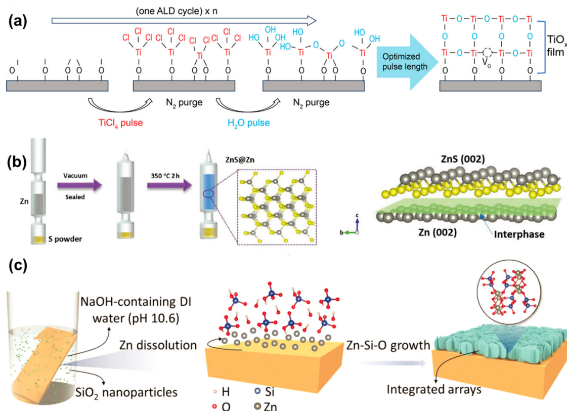
Fig. 9 (a) Illustration of a single ALD cycle with a TiO x coating of thickness of ~0.04 nm. Reproduced from ref. 154 with permission from the American Chemical Society, copyright 2024. (b) Schematic of the artificial ZnS layer preparation. Reproduced from ref. 155 with permission from John Wiley & Sons, copyright 2020. (c) Schematic of the procedure for fabricating the Zn@ZSO composite foil. Reproduced from ref. 156 with permission from John Wiley & Sons, copyright 2022.
