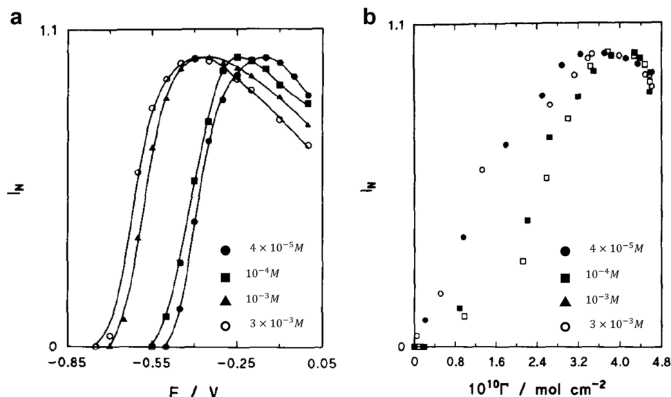
Fig. 50 (a) Plots of the intensity of the 1010 cm⁻¹ band on the electrode potential ( E vs. SCE) for the varied bulk pyridine concentrations. (b) Data from panel a plotted versus surface concentration of pyridine \Gamma . Figures are adapted from ref. 119 with permission. Copyright 1991 Elsevier.
