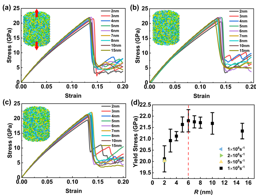
Fig. 2 (a)–(c) Stress–strain curves of sample groups A, B, and C with different R . (d) Variation of yield stress with R , revealing a transition from the HP relation to the IHP relation at R = 6 nm. Simulations on sample group A with R = 2 nm at different strain rates confirm that the deviation of the yield stress obtained with different strain rates remains within the error range.
