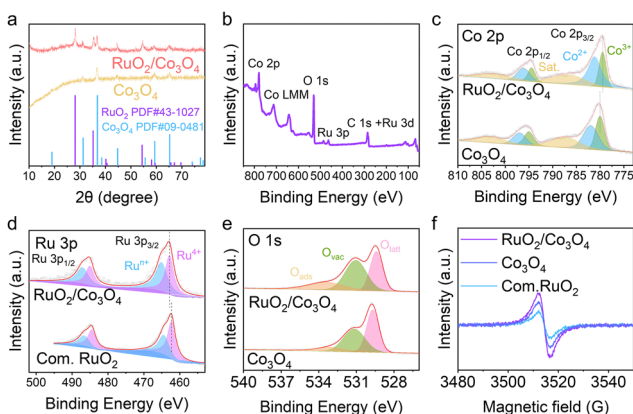
Fig. 3 (a) XRD patterns of \text{RuO}_2/\text{Co}_3\text{O}_4 and \text{Co}_3\text{O}_4 . (b) The whole XPS spectra of \text{RuO}_2/\text{Co}_3\text{O}_4 . (c)–(e) The XPS spectra of (c) Co 2p, (d) Ru 3p, and (e) O 1s for \text{RuO}_2/\text{Co}_3\text{O}_4 . (f) Electron paramagnetic resonance of \text{RuO}_2/\text{Co}_3\text{O}_4 , com. \text{RuO}_2 and \text{Co}_3\text{O}_4 .
