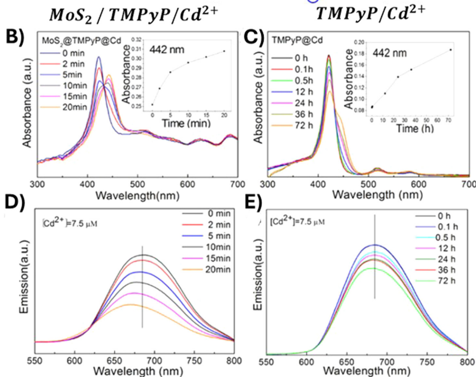
Fig. 43 (A) Schematic showing the strategy for removing \text{Cd}^{2+} using TMPyP self-assembled with \text{MoS}_2 nanosheets. (B) Time-dependent UV-vis absorption spectra of \text{MoS}_2/\text{TMPyP}/\text{Cd}^{2+} and (C) \text{TMPyP} with \text{Cd}^{2+} ; insets: plots of the absorbance at 442 nm versus reaction time. (D) Time-dependent emission spectra of \text{MoS}_2/\text{TMPyP}/\text{Cd}^{2+} and (E) \text{TMPyP}/\text{Cd}^{2+} . Reproduced from ref. 55. Copyright 2017 American Chemical Society.
