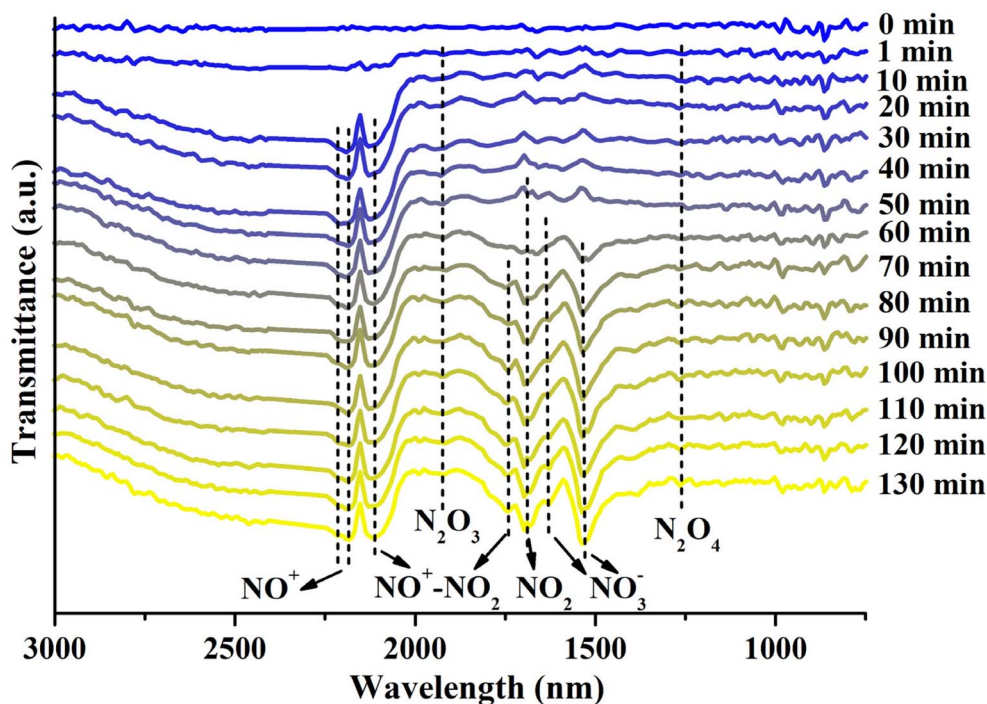
Fig. 6 In situ FTIR spectra of \text{Cu}^{n+}\text{SSZ-13-190-R} during \text{NO}_2 adsorption, with the background of the fresh sample subtracted (conditions: \text{NO}_2 concentration of 1000 ppm, flow rate of 60 \text{ mL min}^{-1} , 25 °C).
