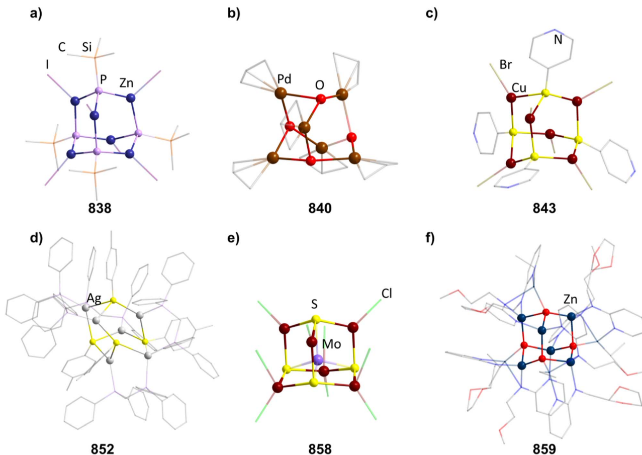
Fig. 18 Examples of adamantane-type cluster with transition metal atoms in the E position: [\text{t}^{\text{Bu}}\text{N}_4]_2[(\text{PSiMe}_3)_4(\text{Zn})_6(\text{thf})_2] ( 838 , top left (a)), [(\text{Pd}\{(\eta^3\text{-C}_3\text{H}_5)\}_4(\text{OH})_6)\text{CF}_3\text{SO}_3] ( 840 , top center (b)), [(4\text{-SC}_5\text{H}_4\text{NH})_4(\text{CuBr})_6] ( 843 , top right (c)), [(\text{SC}_6\text{H}_4\text{Me-p})_4\text{Ag}_6\{(\text{Ph}_2\text{P})_2\text{Me}\}_4][\text{PF}_6]_2 ( 852 , bottom left (d)), [\text{NMe}_4]_5[(\mu_4\text{-Mo})\text{S}_4(\text{CuCl})_3(\text{CuCl}_2)_3] ( 858 , bottom center (e)) and [\text{O}_4(\text{anpy})_8\text{Zn}_6(\text{ZnEt})_4] ( 859 , bottom right (f)). Hydrogen atoms and counterions, if present, are omitted for clarity.
