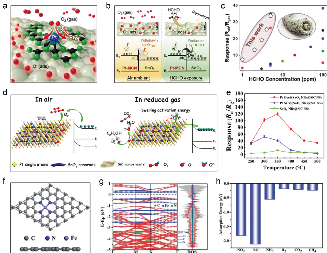
Fig. 5 (a) Schematic illustration of O_2 (gas) dissociation over Pt SAs on Pt-MCN-SnO 2 to form chemisorbed oxygen species ( O_{(ads)}^- ). (b) Schematic illustration showing the HCHO-sensing mechanism as well as the simplified energy band diagram of the heterojunction between MCN and SnO 2 . (c) Comparison of the state-of-the-art formaldehyde gas sensors with that made of Pt-MCN-SnO 2 . Reproduced with permission from ref. 127 Copyright 2020, American Chemical Society. (d) Schematic illustration showing the gas sensing mechanism of Pt SAs@SnO 2 NRs@SiC NSs. (e) Gas sensing response toward 500 ppm ethanol versus operating temperature over Pt SAs@SnO 2 NRs@SiC NSs, Pt NCs@SnO 2 NRs@SiC NSs, and SnO 2 NRs@SiC NSs. Reproduced with permission from ref. 128 Copyright 2020, American Chemical Society. (f) Top and side views showing the atomic configuration of FeNC in a 5 × 5 supercell. (g) Electronic band structure and density of states (DOS) for FeNC. (h) Adsorption energies of NO 2 , NO, NH 3 , H 2 , CO 2 and CH 4 on FeNC. Reproduced with permission from ref. 129 Copyright 2020, Royal Society of Chemistry.
