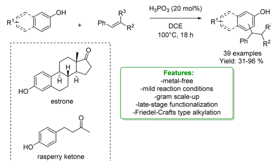
Scheme 19 \text{H}_3\text{PO}_3 -catalysed alkylation of phenols with alkenes. 85
