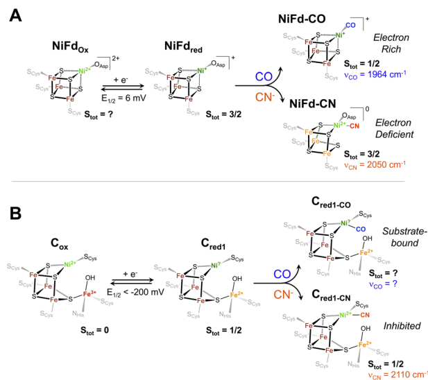
Fig. 8 Proposed electronic and geometric structures of the (A) NiFd ox , NiFd red , NiFd-CO, and NiFd-CN species with key experimental metrics indicated that have been obtained from this work, and (B) analogous C ox , C red1 , C red1 -CO, and C red1 -CN states of CODH with spectroscopic metrics obtained from ref. 17, 75 and 76.
