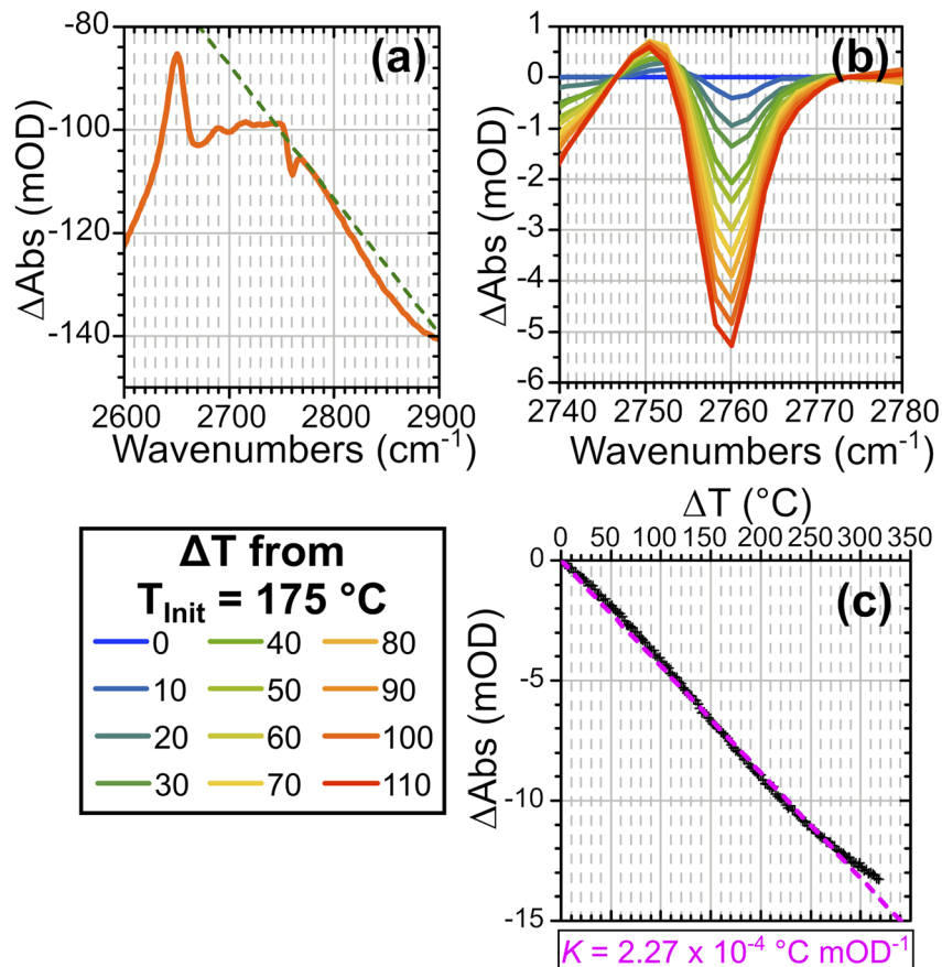
Fig. 5 (a) FTIR difference spectrum of \Delta T = 50\text{ }^\circ\text{C} from T_{\text{init}} = 175\text{ }^\circ\text{C} showing a linear baseline fit to isolate silanol mode contributions. (b) Comparison of the \nu(\text{SiOD}) feature in baseline subtracted difference spectra at indicated \Delta T values showing increase in intensity of negative feature with increased \Delta T . (c) Variation of \nu(\text{SiOD}) negative intensity with \Delta T showing linear relationship with slope 1/K .
