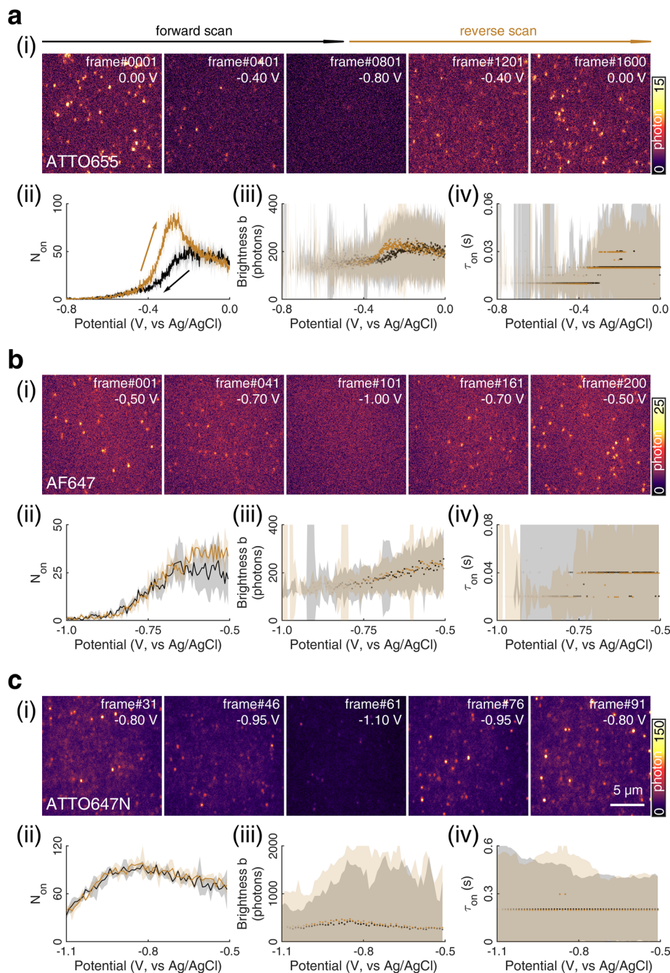
Fig. 1 (i) SM-EC imaging of (a) ATTO655, (b) AF647, and (c) ATTO647N dye molecules on nanoporous ATO (nATO) films in 1 M \text{NaNO}_3 solution while sweeping the applied electrochemical potential (see Movies S1–S3† for full videos). The (ii) number N_{\text{on}} , (iii) brightness b , and (iv) duration \tau_{\text{on}} of single-molecule fluorescence bursts captured during the potential sweeps. The (ii) solid line and (iii) and (iv) dots represent the median values and the shaded areas represent \pm 1 standard deviation of response over three full sweep cycles. Black and dark yellow trajectories represent the forward and reverse scans, respectively. Scale bar: 5 \mu\text{m} .
