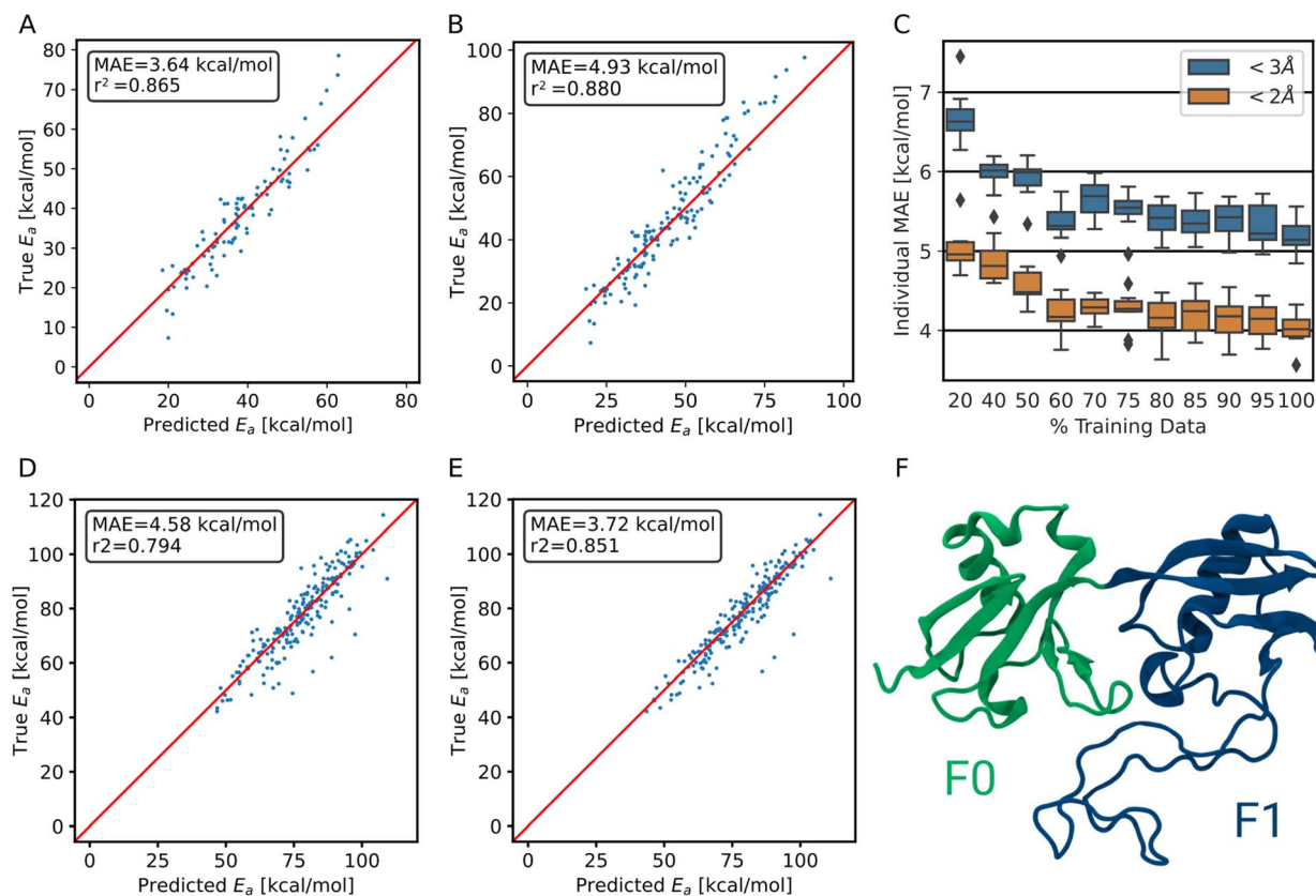
Fig. 5 Performance of the transfer-learned ensemble model on (A) trajectory test data <2 \text{ \AA} and on (B) <3 \text{ \AA} trajectory test data. (C) Learning curve of the transfer learning process. The test MAE of the individual models is shown. (D) Performance of the ensemble model trained on synthetic and collagen-trajectory data on the F0F1 domain of FERM. (E) Ensemble model performance after transfer learning on as little as 500 structures of FERM on same evaluation set as in D. (F) The F0 and F1 domain of FERM used in out-of-domain predictions. It includes \alpha -helices, \beta -sheets and an intrinsically disordered region.
