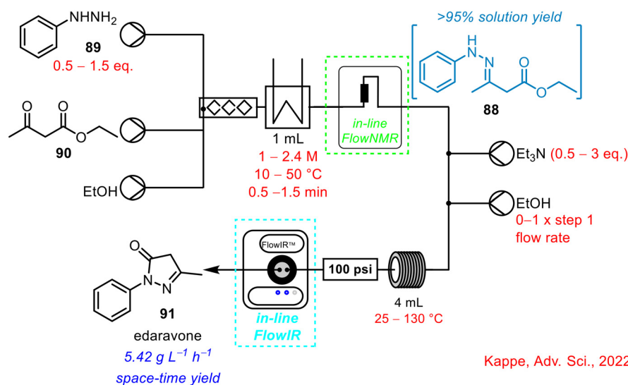
Scheme 35 Telescoped two-step synthesis of API edavarone using in-line FlowNMR to monitor initial imine formation step. 76
