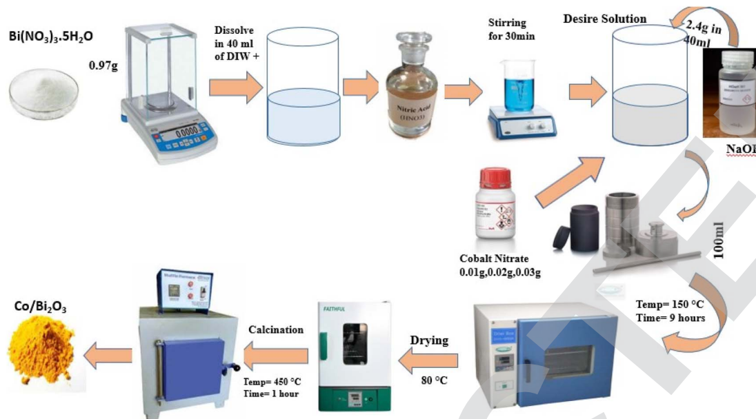
Fig. 1 Hydrothermal synthesis of cobalt-doped bismuth oxide nanoparticles.
