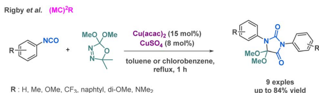
Scheme 4 Synthesis of hydantoin derivatives by Rigby et al.
