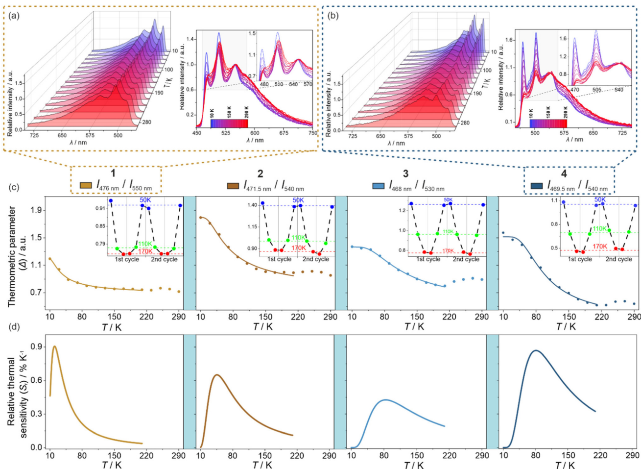
Fig. 5 Luminescent thermometry characteristics of 1–4 , including the sets of temperature-variable normalized emission spectra under the 400 nm excitation for 1 (a) and 4 (b), presented by a 3-D plot as well as by overlapped spectra at indicated temperatures (the comparison of data for all compounds is provided in Fig. S13–S16†), the temperature dependences of selected thermometric parameters (c) (defined as the ratios between indicated emission wavelengths), shown with the repeatability cycles of thermometric behavior (the insets), and the resulting relative thermal sensitivity curves (d). In (c), filled points are experimental data while solid lines represent the best-fit curves following eqn (1).
