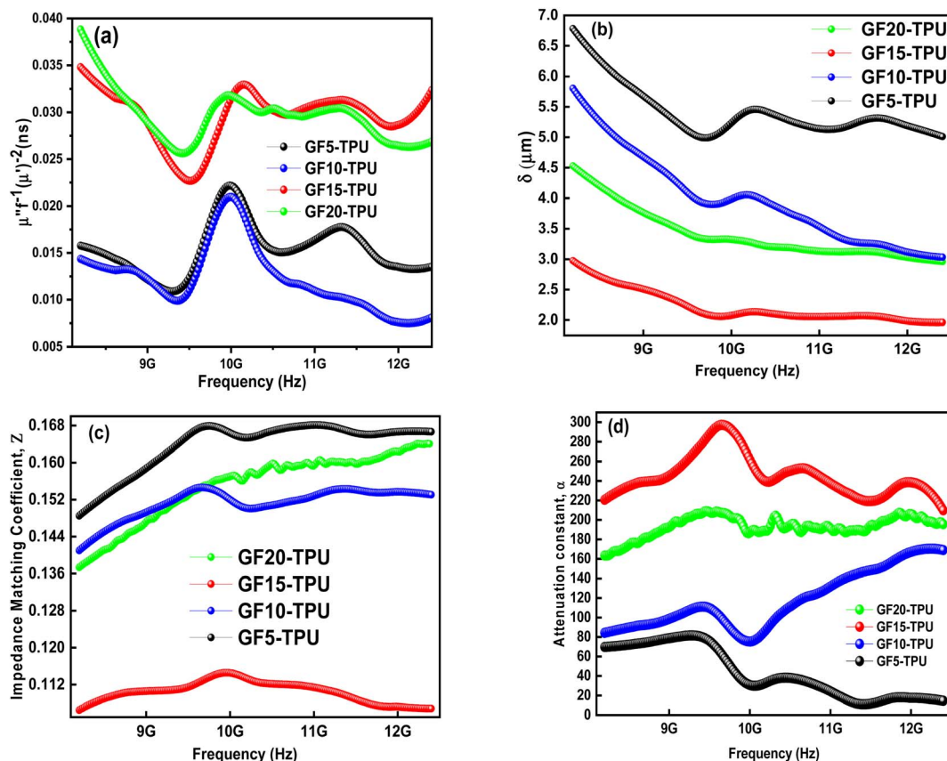
Fig. 11 Variation of (a) eddy current loss, C_{\omega} , (b) skin-depth, \delta , (c) impedance matching coefficient, Z , and (d) attenuation constant, \alpha , as a function of the frequency for all the developed GF-TPU nanocomposites.
