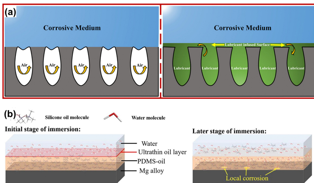
Fig. 15 Corrosion prevention mechanism of (a) SHSs and SLIPSS (reproduced from ref. 188 with permission from [Wiley], copyright [2021]) and (b) organogel (reproduced from ref. 189 with permission from [Elsevier], copyright [2021]).
