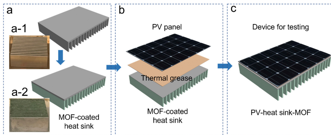
Fig. 2 Schematic of device assembly processes. (a) the MOF coating process; (a-1) photo of the heat fins before spray coating; (a-2) photo of the heat fins after spray coating with Cr- soe -MOF-1. (b) The device assembling process. (c) The as-assembled devices for testing.
