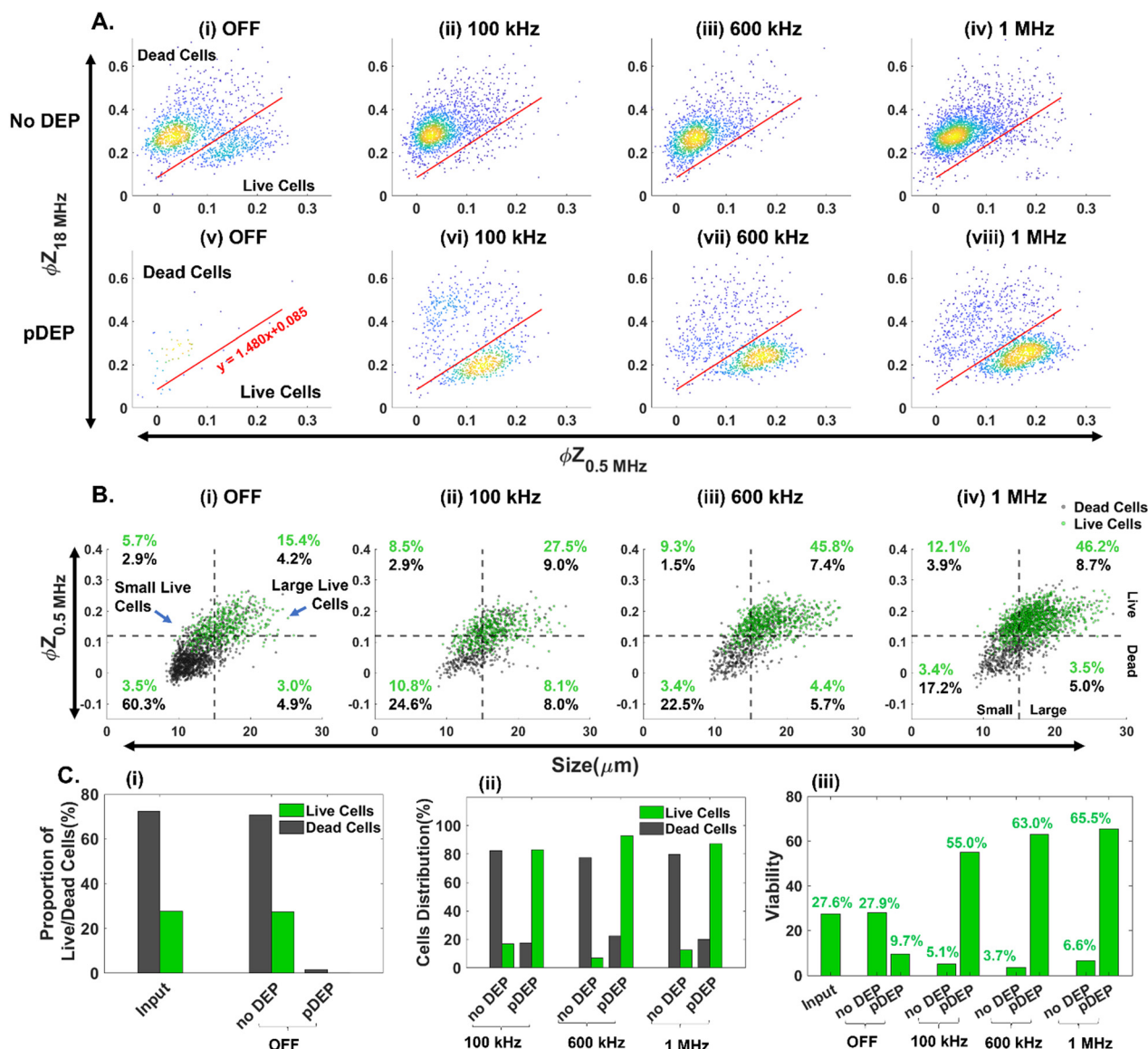
Fig. 4 Using impedance cytometry to optimize the frequency for pDEP enrichment (at 25 V_{pp} ) of live cells over the entire size range of an input sample (~27% live PDAC cells). Single-cell impedance scatter plots of: A) \phi Z_{18\text{ MHz}} vs. \phi Z_{0.5\text{ MHz}} for live cell gating of the sample from “pDEP” and “no DEP” outlets; and B) \phi Z_{0.5\text{ MHz}} vs. electrical size for size-stratified live vs. dead cells in the input and pDEP outlets post-DEP. C) Quantifying collection at the “pDEP” and “no DEP” outlets (25 V_{pp} at 0.1–1 MHz) based on: (i) proportion of live and dead cells; (ii) cell distribution in each outlet at different DEP trapping frequencies and (iii) viability of collected cells. All live vs. dead cell gates (lines in 2D plots) are obtained based on the optimized hyperplane from the SVM supervised learning model.
