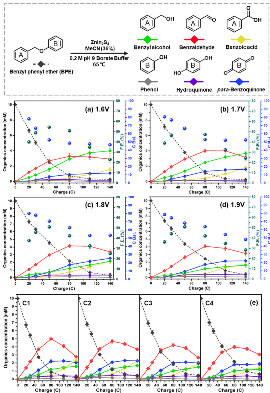
Fig. 6 Electrolysis of BPE using the R-ZIS electrode in pH 9 buffer solutions at (a) 1.6 V, (b) 1.7 V, (c) 1.8 V, and (d) 1.9 V_{\text{Ag}/\text{AgCl}} in 65 °C. (e) Formation of products in four stability cycle tests in pH 9 buffer solutions at 2 V_{\text{Ag}/\text{AgCl}} in 65 °C.
