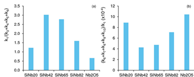
Fig. 4 Ratio of rate constants (a) reflecting favourable C8 formation (higher ratio k_1/(k_3 + k_4 + k_5 + k_9) ), or (b) enhanced decomposition paths to byproducts (higher ratio (k_6 + k_7 + k_8 + k_9 + k_{10})/k_1 ). Reaction conditions: 1.6 M Fur in acetone, 140 °C, 29.7 \text{g}_{\text{cat}} \text{L}^{-1} .
