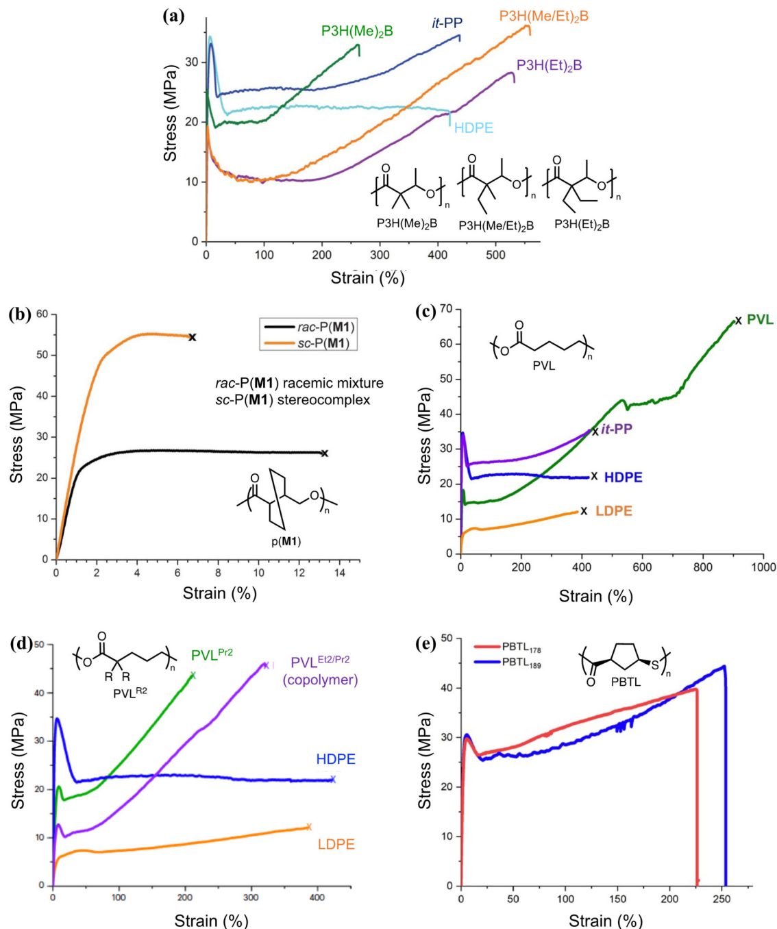
Fig. 6 A side-by-side comparison of the tensile curves of various circular polyesters, polythioester, in comparison to isotactic polypropylene ( it -PP), high-density polyethylene (HDPE), and low-density polyethylene (LDPE). Details about their syntheses and recycling properties are shown in Fig. 5. (a) is reproduced from ref. 63 with permission from AAAS, copyright 2023. (b) is reproduced from ref. 64 from AAAS, copyright 2018. (c) is reproduced from ref. 65 with permission from Wiley, copyright 2023. (d) is reproduced from ref. 66 with permission from Springer Nature, Copyright 2023. (e) is reproduced from ref. 67 with permission from AAAS, copyright 2020.
