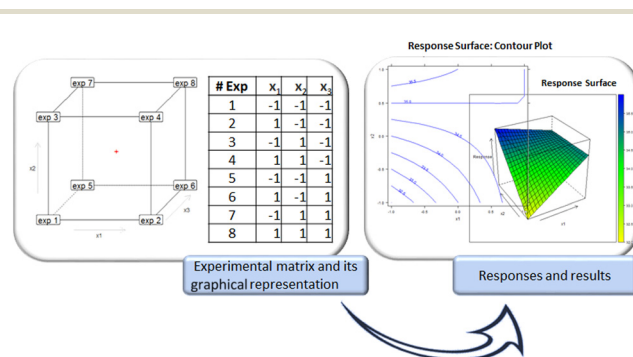
Fig. 2 Different steps characterizing the DoE approach. The example refers to a full factorial design.
