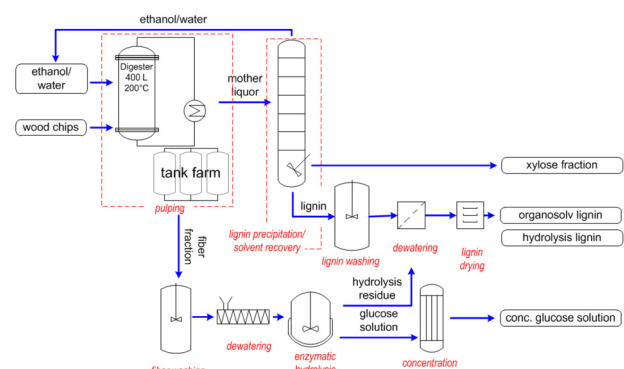
Fig. 6 Example of the Fraunhofer Centre organosolv process (reproduced with permission and courtesy from Fraunhofer CBP, copyright: © Fraunhofer CBP).
