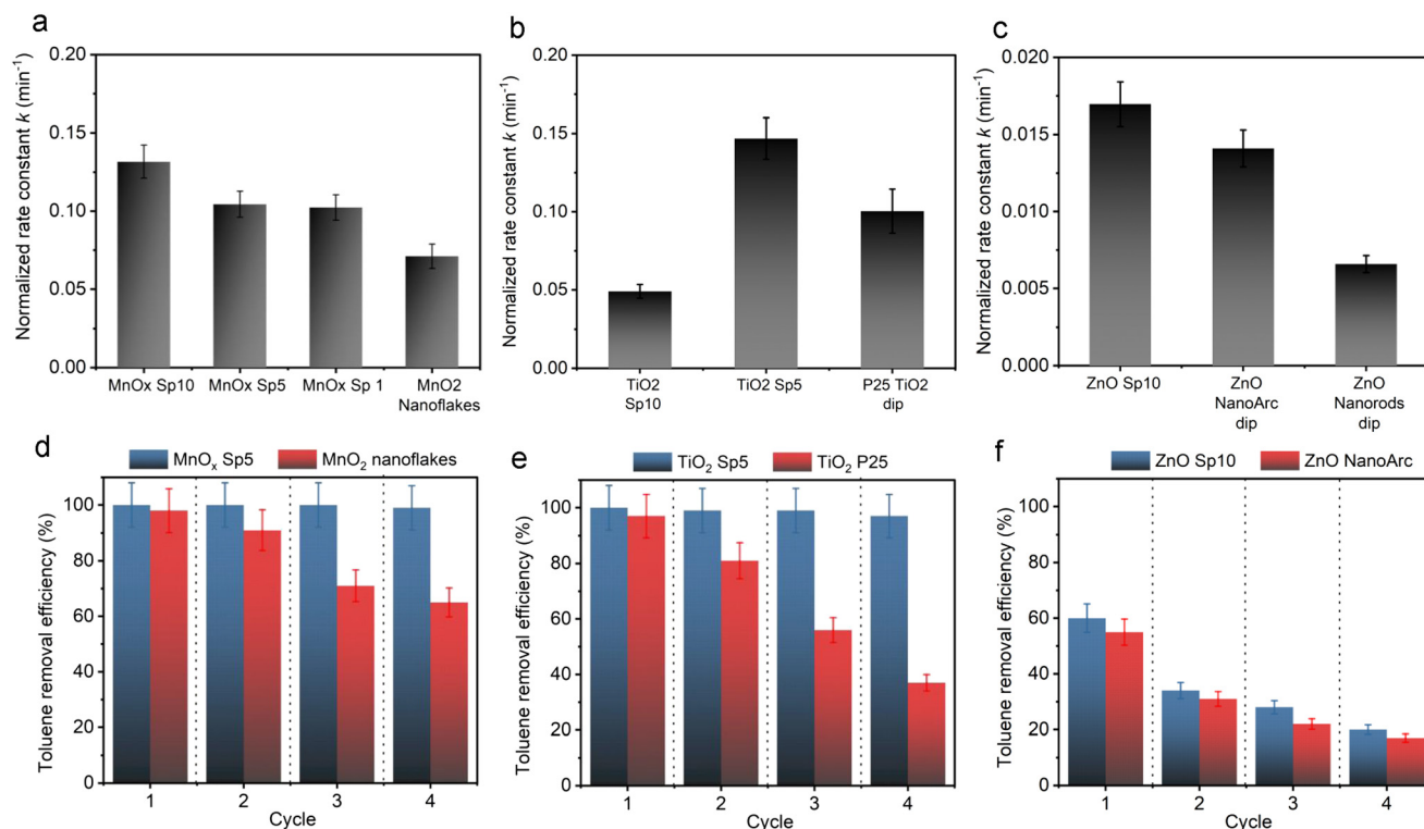
Fig. 12 Normalized 1st order reaction rate constant k for a) spark-ablated manganese oxide (Mn x Sp) nanoparticles and MnO 2 nanoflakes, b) spark-ablated and commercial titanium dioxide (TiO 2 Sp and TiO 2 P25), and c) spark-ablated and commercial zinc oxide (ZnO Sp10 and ZnO NanoArc) nanoparticles. Photocatalyst stability over four consecutive toluene degradation cycles represented as toluene removal efficiency after 60 min of irradiation for d) MnO x Sp and MnO 2 nanoflakes, e) TiO 2 Sp5 and TiO 2 P25, and f) ZnO Sp10 and ZnO NanoArc nanoparticles.
