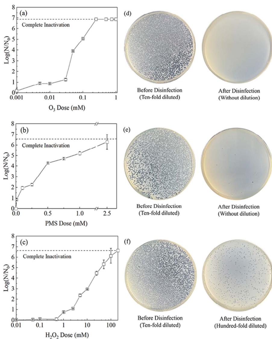
Fig. 1 Inactivation efficiency of MS2 coliphage in 30 min with different oxidants (a) O 3 (0.001–1 mM), (b) PMS (0.01–2.5 mM), (c) H 2 O 2 (0.01–200 mM); (d–f) culture plates of MS2 coliphage treated with 1 mM (d) O 3 , (e) PMS, and (f) H 2 O 2 .
