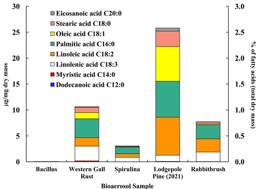
Fig. 4 Fatty acid concentration (in \mu\text{g} per \text{mg} dry mass) of selected bioaerosols. The secondary axis shows the percentage of fatty acids per milligram of dry mass. Fatty acids in Bacillus were below detection limit. Standard deviations range from 0.006 \mu\text{g mg}^{-1} in eicosanoic acid (spirulina) to 1.03 \mu\text{g mg}^{-1} in palmitic acid (lodgepole pine 2021) (see Table S4† for details).
