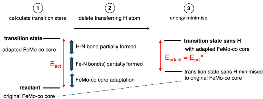
Scheme 1 Components of the calculated activation potential energy for a reaction in which an H–N bond is formed, and the procedure for calculation of the activation energy E_{\text{act}}^* excluding the H–N bond formation component.
