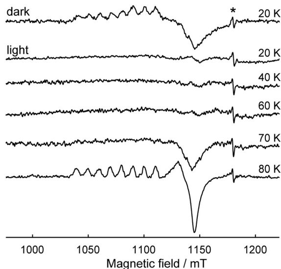
Fig. 6 Left: LIESST experiment on the [\text{Fe}(\mu\text{-bpp})_2][\text{BF}_4]_2 host lattice. The sample was cooled to 10 K then irradiated with green light, causing photoexcitation to its high-spin state which is metastable at those temperatures. 20,21,26 Rewarming to 80 K leads to thermal high \rightarrow low spin relaxation. Right: Q-band EPR spectra of [\text{Fe}(\mu\text{-bpp})_2]_{0.97}[\text{Co}(\text{terpy})_2]_{0.03}[\text{BF}_4]_2 under LIESST conditions. The sample was measured prior to illumination (20 K, dark); irradiated and remeasured (20 K, light); then warmed at 10 K intervals up to its high \rightarrow low relaxation temperature. The asterisk marks a radical impurity. This figure has been adapted from ref. 28 with permission from the Royal Society of Chemistry, copyright 2006; and from ref. 102 with permission from the American Chemical Society, copyright 2018.
