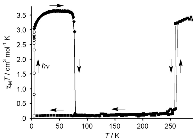
Fig. 6 Left: LIESST experiment on the [\text{Fe}(\mu\text{-bpp})_2][\text{BF}_4]_2 host lattice. The sample was cooled to 10 K then irradiated with green light, causing photoexcitation to its high-spin state which is metastable at those temperatures. 20,21,26 Rewarming to 80 K leads to thermal high \rightarrow low spin relaxation. Right: Q-band EPR spectra of [\text{Fe}(\mu\text{-bpp})_2]_{0.97}[\text{Co}(\text{terpy})_2]_{0.03}[\text{BF}_4]_2 under LIESST conditions. The sample was measured prior to illumination (20 K, dark); irradiated and remeasured (20 K, light); then warmed at 10 K intervals up to its high \rightarrow low relaxation temperature. The asterisk marks a radical impurity. This figure has been adapted from ref. 28 with permission from the Royal Society of Chemistry, copyright 2006; and from ref. 102 with permission from the American Chemical Society, copyright 2018.
