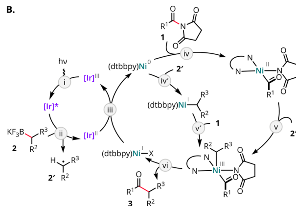
Scheme 15 Key early development in Ni-catalysed acylative coupling using a C(acyl)-N electrophile with dual photoredox and Ni catalysis.
