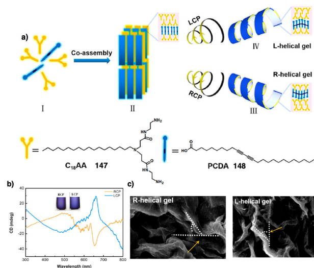
Fig. 70 (a) Structures 147 and 148 and schematic illustration of the asymmetry induction by CP-light irradiation of 147 – 148 co-assembly. (b) ECD spectra showing opposite chirality after irradiation with L / R CP-light. (c) SEM images of the gels with different handedness. Reproduced from ref. 347 with permission from the American Chemical Society, copyright 2022.
