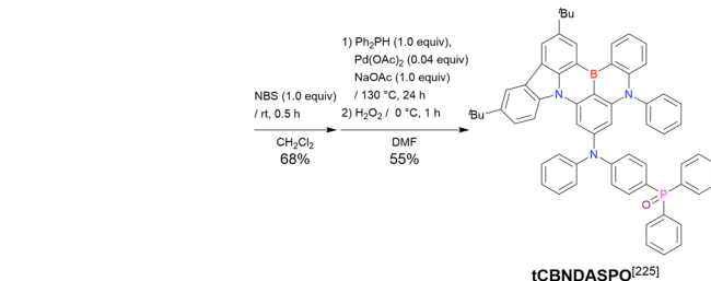
Scheme 50 Late-stage introduction of sulfoxide, sulfone, and phosphine oxide groups.
